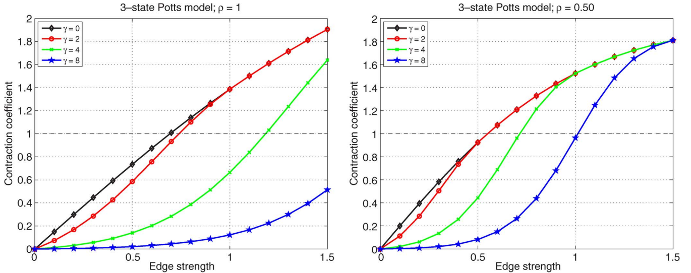
Fig. 5. Illustration of the benefits of observations. Plots of the contraction coefficient from Corollary 9 versus the edge strength for a 3-state Potts model. Each curve corresponds to a different setting of the SNR parameter \gamma . (a) Ordinary sum-product algorithm \rho = 1 . Upper-most curve labeled \gamma = 0 corresponds to the best bounds from previous work [10], [11], [20]. (b) Reweighted sum-product algorithm \rho = 0.50 .
