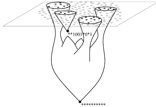
FIG. 1. The set of fully assigned satisfying configurations occupy the top plane, and are arranged into clusters. Enlarging to the space of partial assignments leads to a new space with better connectivity. Minimal elements in the partial ordering are known as cores. Each core corresponds to one or more clusters of solutions from the top plane. In this example, one of the clusters has as a core a non-trivial partial assignment, whereas the others are connected to the all-* assignment.
