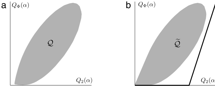
Fig. 3. Geometry of the proof of (17). Display (a) is a plot of the set Q := \{(Q_2(\alpha), Q_\Phi(\alpha)) : \|\alpha\|_{\ell_2} = 1\} \subset \mathbb{R}^2 . This is a convex set as a consequence of Hausdorff–Toeplitz theorem on convexity of the numerical range and preservation of convexity under projections. Display (b) shows the set \tilde{Q} := \text{conv}(0, Q) , i.e., the convex hull of \{0\} \cup Q . Observe that R_\Phi(\varepsilon) = \sup\{x : (x, y) \in \tilde{Q}, y \leq \varepsilon^2\} . For any fixed \rho^2 \in (0, 1) , the bound is a piecewise linear approximation (in \varepsilon^2 ) to one side of \tilde{Q} as shown in display (b).
