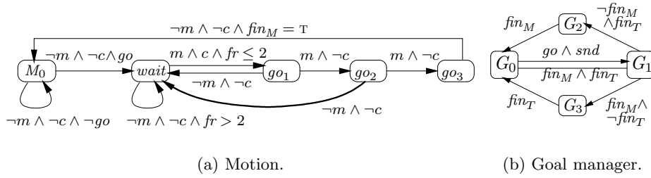
Fig. 2. A/G interfaces modeling a Lego robot.
