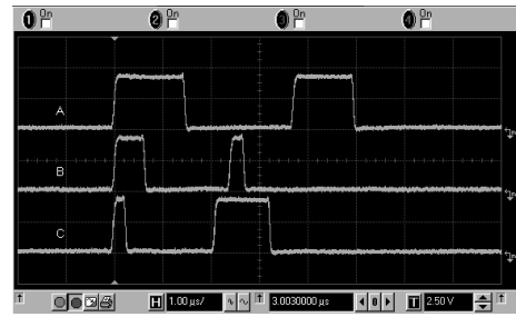
Figure 17: Context Switching on an Oscilloscope
