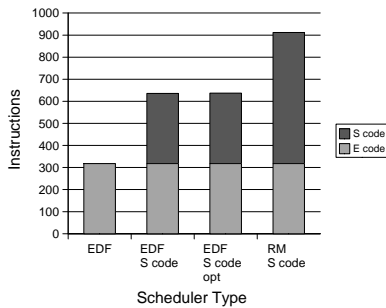
Figure 18: E and S code size for 100 tasks
