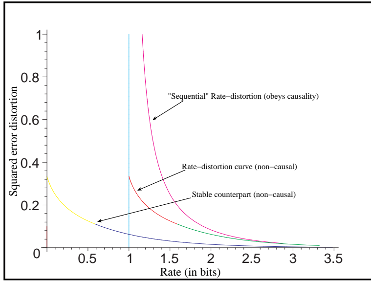
Fig. 4. The distortion-rate curves for an unstable Gauss-Markov process with \lambda = 2 and its stable backwards-version. The stable and unstable D(R) curves are related by a simple translation by 1 bit per symbol.
