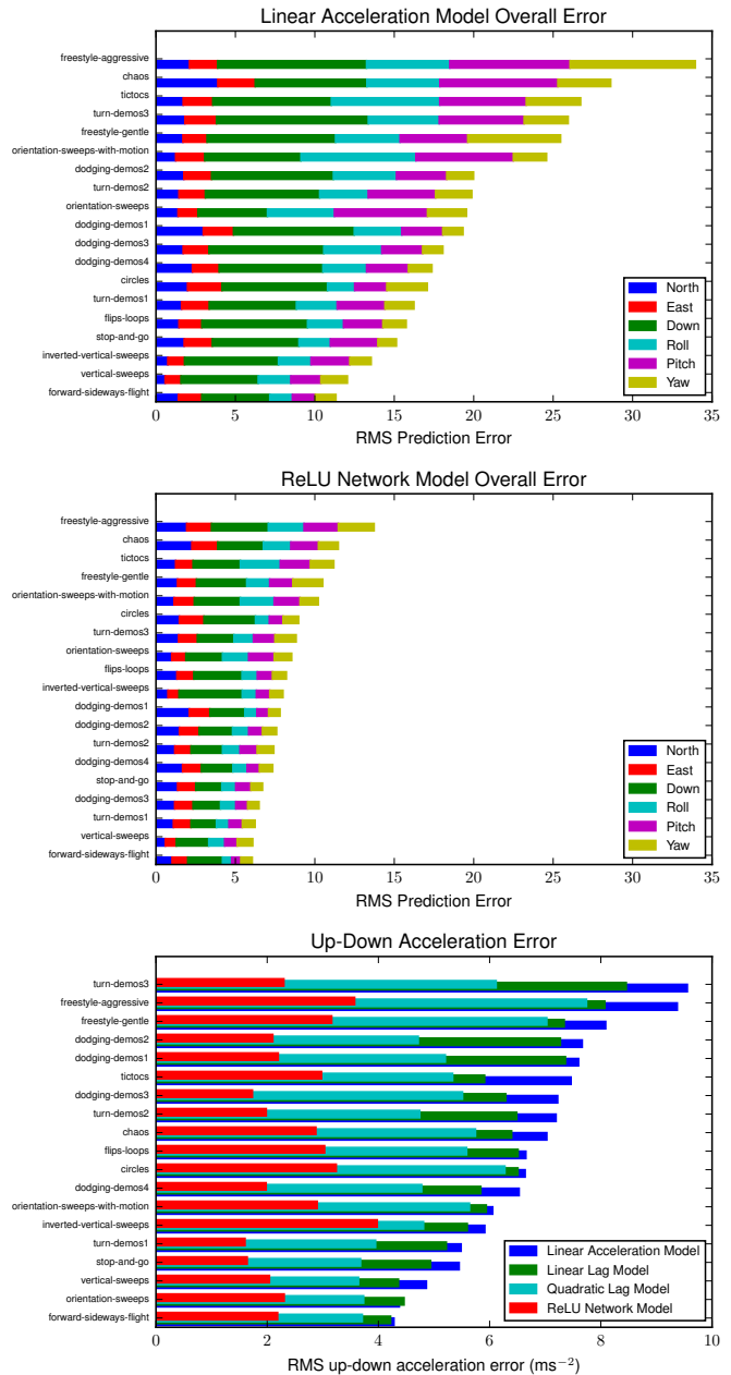
Fig. 5. Performance Comparison of the ReLU Network Model and baseline models from Section III. Top: Overall RMS prediction error of the Linear Acceleration Model over all acceleration components, each denoted by a different color. Middle: Overall RMS prediction error of the ReLU Model over all acceleration components. Across all maneuvers, this result represents a 58% improvement in RMS error over the Linear Acceleration Model above. Bottom: RMS Error in predicting the up-down acceleration of the helicopter on test-set trajectories, which is empirically found to be the most difficult component to predict. The Linear Acceleration Model (blue) is outperformed successively by the Linear Lag Model which accounts for control lag, and the Quadratic Lag Model which accounts for some simple nonlinearities. The ReLU Network Model significantly outperforms all baselines, demonstrating the importance of accounting for hidden system state. Performance is displayed separately for each maneuver, but the labels are not used during training. Across all maneuvers, the ReLU Network Model reduces up-down RMS error of the Linear Acceleration Model by 60% . Note that the Linear baseline models actually correspond to nontrivial nonlinear dynamics models (see Section III).
