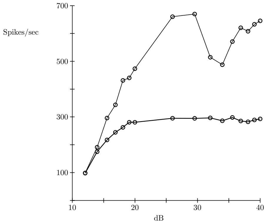
Figure 4. Instantaneous firing rate of the adaptive neuron, as a function of amplitude (in dB). Top curve is firing rate at onset of response, bottom curve is firing rate after adaptation. Tone burst frequency is 1KHz.
