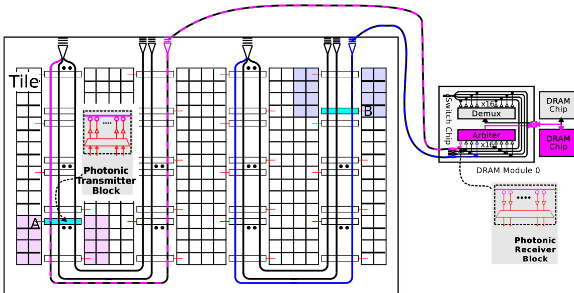
Figure 3: LMGs network design for a 64-tile system with 16 groups implemented using a u-shaped physical network. Two different requests to the same DRAM are highlighted.
