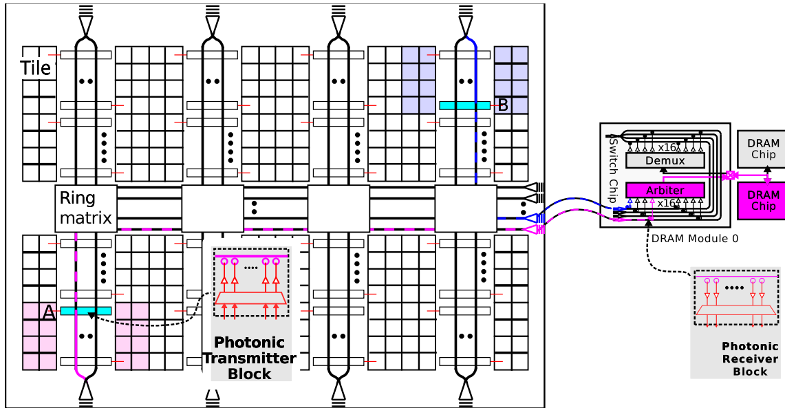
Figure 2: LMGs network design for a 64-tile system with 16 groups implemented using a ring matrix physical network. Two different requests to the same DRAM are highlighted.
