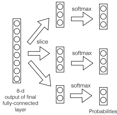
Figure 5: Computation of factored discrete probability distribution in Atari domain
