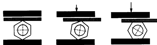
Figure 7: Time-sequence of grasping with the modified gripper. (1) As the two outer jaws close over a typical part (hex nut), horizontal forces cause the sliding jaw to translate to the left (2) until the part is gripped in a stable configuration (3). (Based on drawing by Ben Brown).
