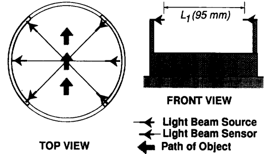
Figure 1: The usual cross-beam sensor configuration
