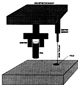
Figure 10: An instrumented gripper
