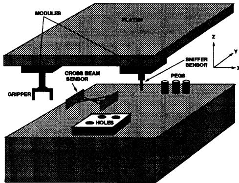
Figure 9: The RobotWorld multi-robot system
