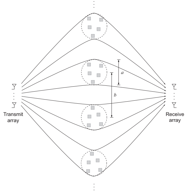
Fig. 9. A physical environment with an infinite line of scattering clusters in the midway between transmitter and receiver.
