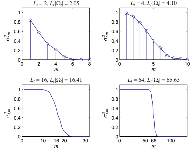
Fig. 6. Plots \sigma_{t,m}^2 for \Theta_t = [25^\circ, 55^\circ] \cup [80^\circ, 110^\circ] \cup [145^\circ, 175^\circ] ( |\Omega_t| = 1.0254 ) and L_t varying from 2 to 64.
