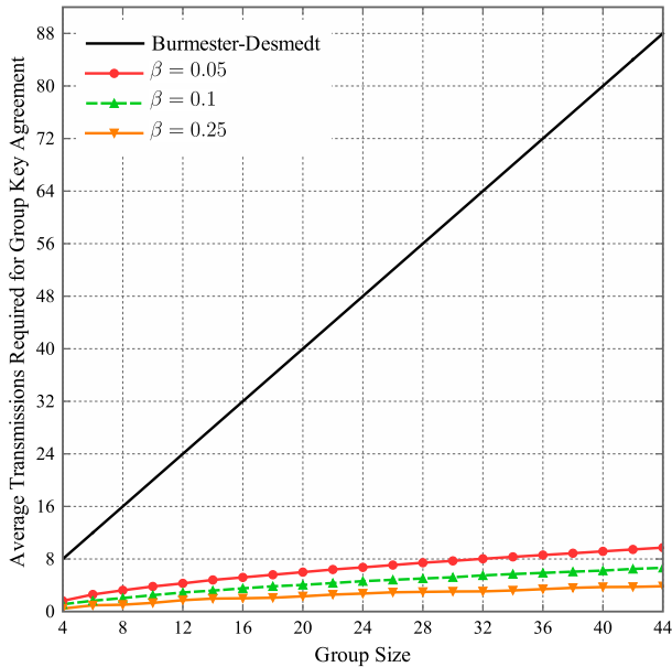
Fig. 4. Number of public multicast transmissions required for group key agreement via the proposed protocol when \lceil 50/\beta \rceil master keys are loaded randomly in a 50-client network. Our protocol exhibits a sublinear growth in the number of transmissions as the group size increases.
