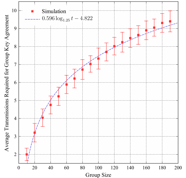
Fig. 5. Number of public multicast transmissions for group key agreement for the proposed protocol when n = 200 , R = 100 , \beta = 0.2 , and b = 1.25 . The number of transmissions required for key agreement grows as the logarithm of the group size.
