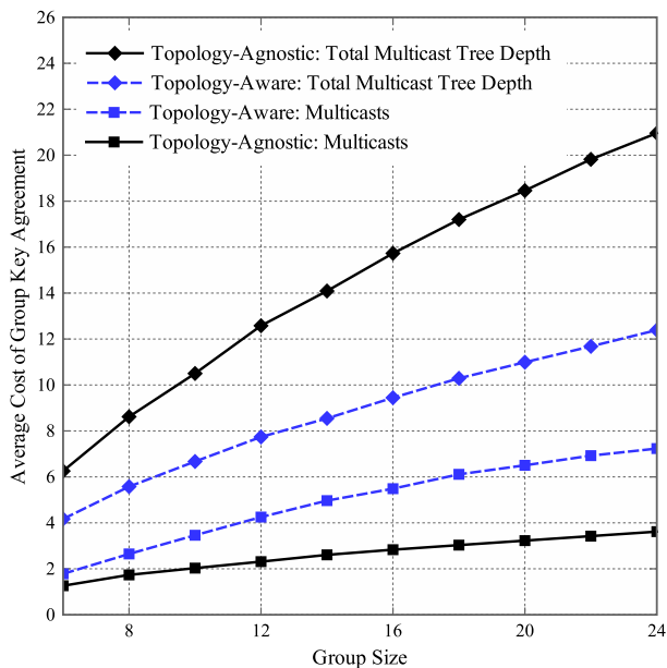
Fig. 8. Average cost of group key agreement of the topology-agnostic (Algorithm 1) and topology-aware (Algorithm 2) variants of our protocol in an n = 100 client network.
