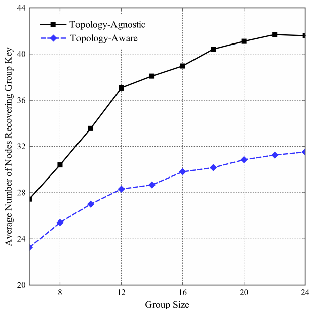
Fig. 9. Average number of clients that can recover the group key as a function of the group size in the topology-agnostic and topology-aware protocols. By constraining the tree-depth of each multicast transmission, fewer unintended clients can recover the group key under the topology-aware variant.
