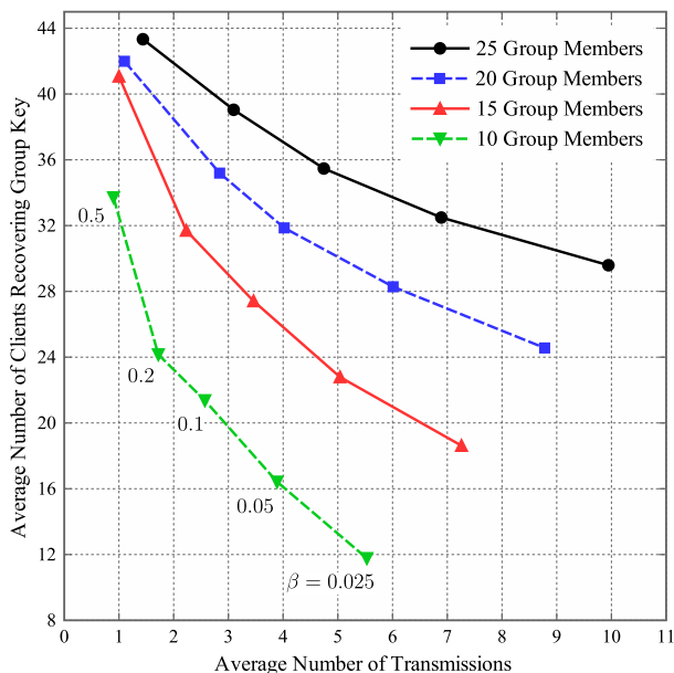
Fig. 6. The average number of clients that can recover the group key as a function of the average number of transmissions required to generate it. The tradeoffs illustrated here, along with the likelihood that a compromised node goes undetected, can inform master key loading scheme parameter selection.
