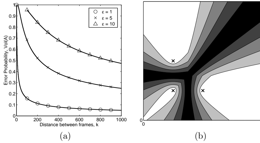
Figure 3: (a) The error probability for the hamming cube at different values of \epsilon and distances k between the frames in the video. (b) Values of ranking function Q(\cdot) for a three-frame video sequence. Lighter colors correspond to larger values.
