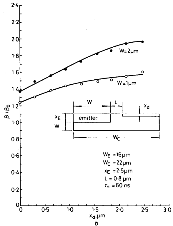
Fig. 3B Normalised current gain of vertical n-p-n transistor as a function of the depletion-layer width X_d for two different base widths
