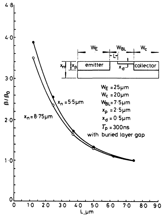
Fig. 6 Normalised current gain of lateral p-n-p transistor as a function of the spacing L between the emitter edge and field plate for two values of epilayer thickness X_n
