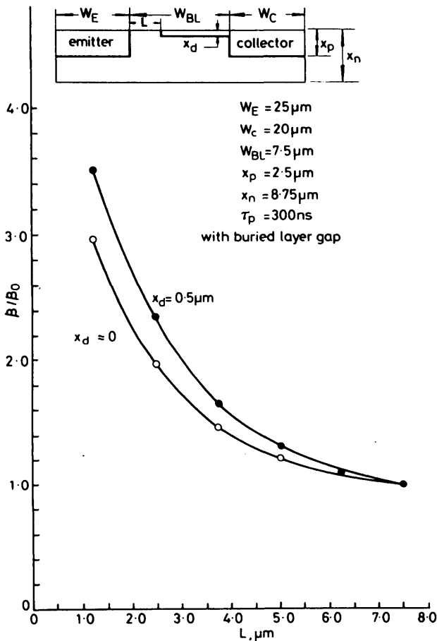
Fig. 5 Normalised current gain of lateral p-n-p transistor as a function of the spacing L between the emitter edge and the field plate for two values of the depletion layer width X_d
