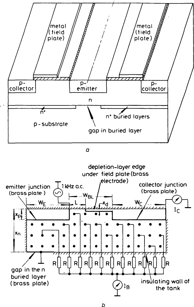
Fig. 2 Lateral p-n-p transistor
