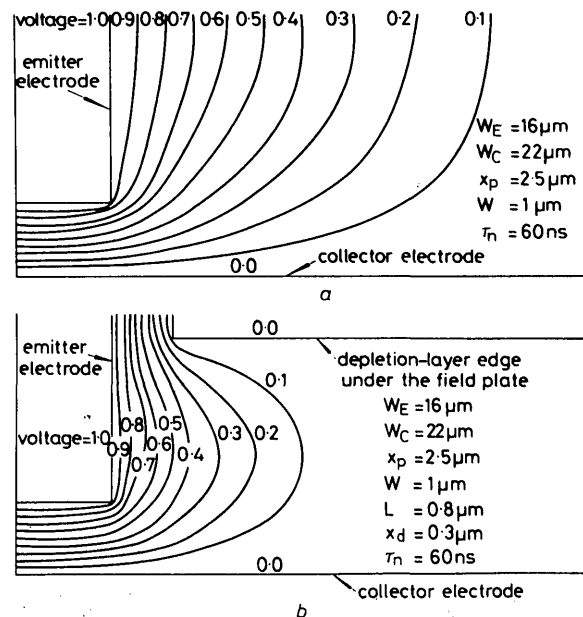
Fig. 4 Minority-carrier density distribution in the base region of vertical n-p-n transistor
