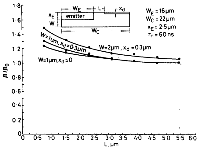
Fig. 3A Normalised current gain of vertical n-p-n transistor as a function of the separation L between the field plate and the emitter-base edge for different values of the depletion-layer width X_d and base width W
