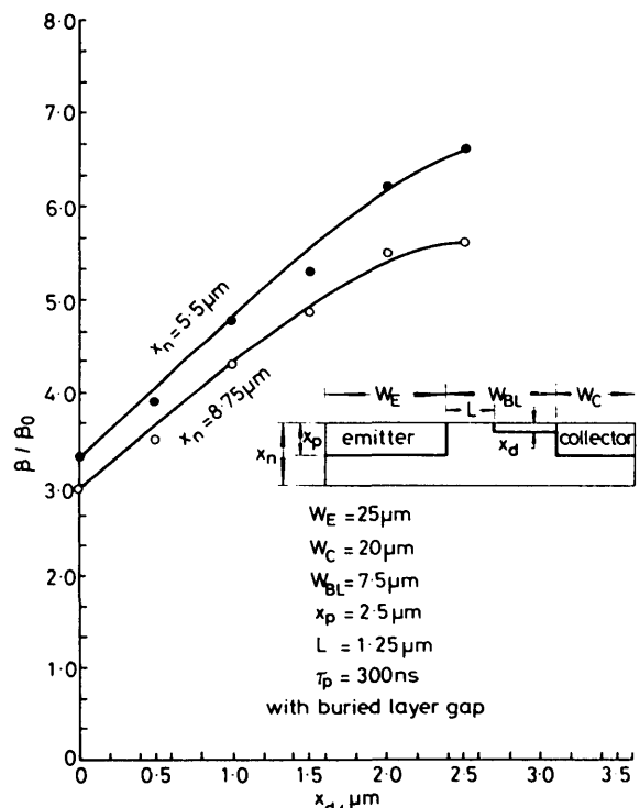
Fig. 7 Normalised current gain of lateral p-n-p transistor as a function of the depletion layer width X_d under the field plate for two values of the epilayer thickness X_n
