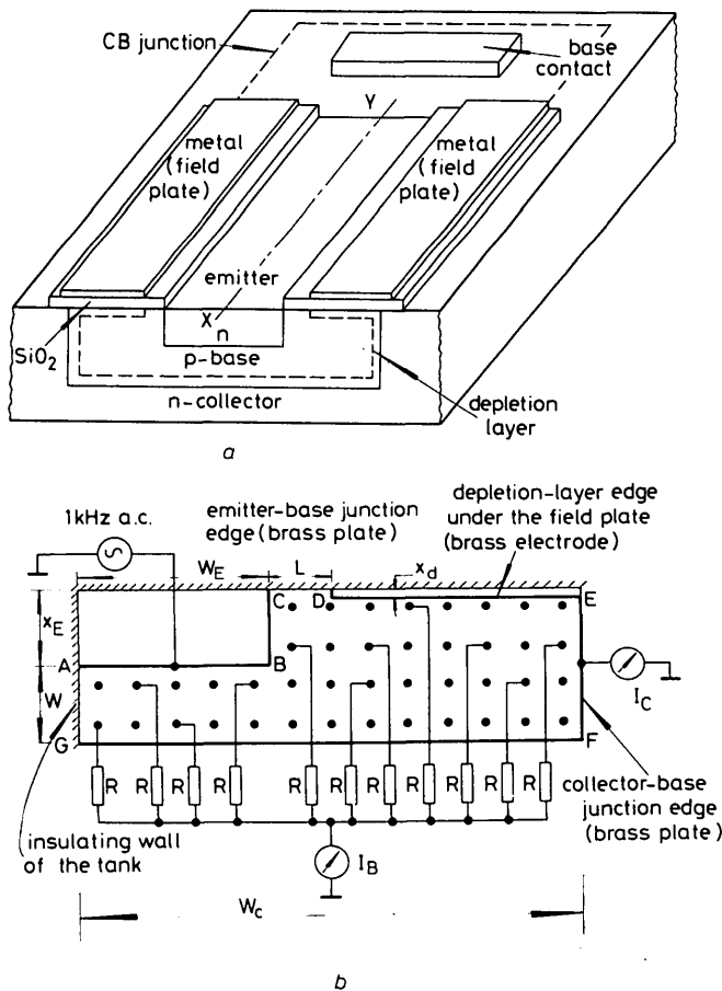
Fig. 1 Vertical n-p-n transistor
