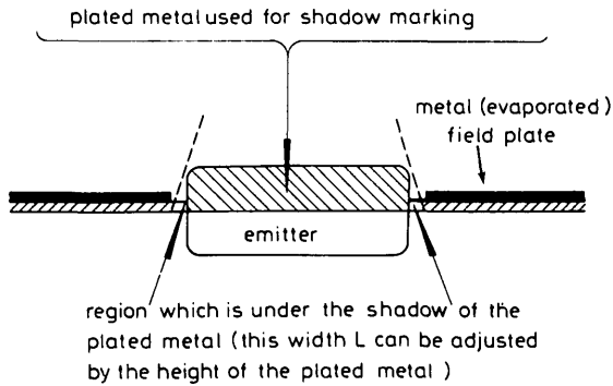
Fig. 8 Electroless plated metal on the emitter for using as a shadow mask during evaporation of metal for the field plate.
