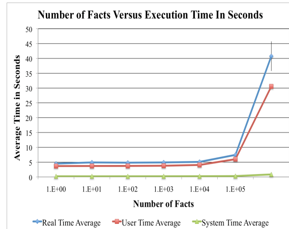
Graph 4 - Drools rule engine simple performance test results
