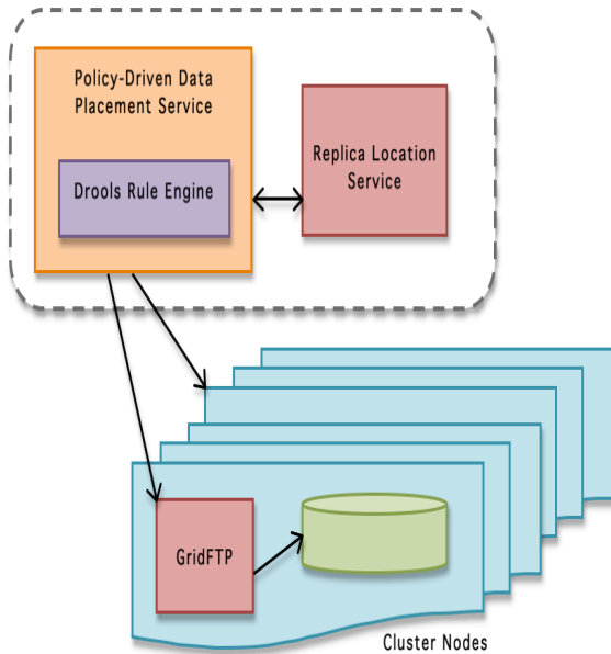
Figure 1 - High-level architecture of the Policy-Driven Data Placement Service
