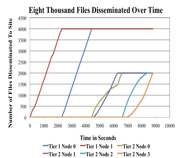
Graph 3 - Dissemination policy execution time using eight thousand files
